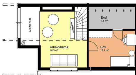
PLAN 2
